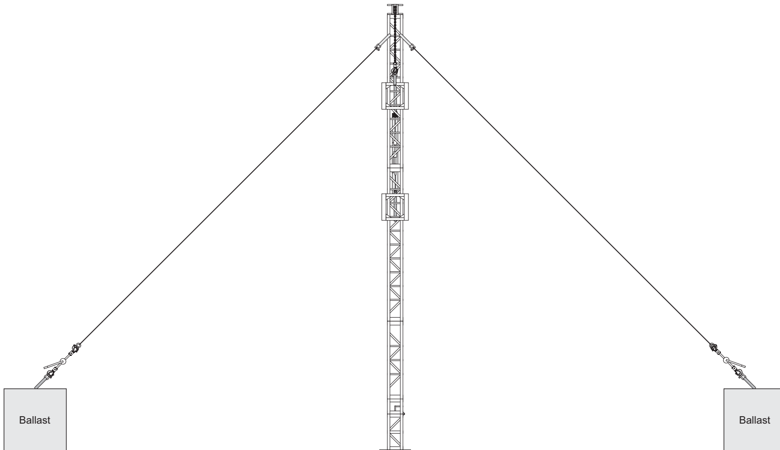
Side View
